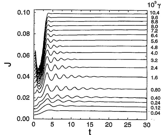
FIG. 8. Evolution of the PC J for different values of the photogeneration \gamma (in units of 10^{-3} ), which increases from bottom to top of the figure, as indicated at the right margin. The voltage ( \phi = 1.1 ) is the same for all the curves.
