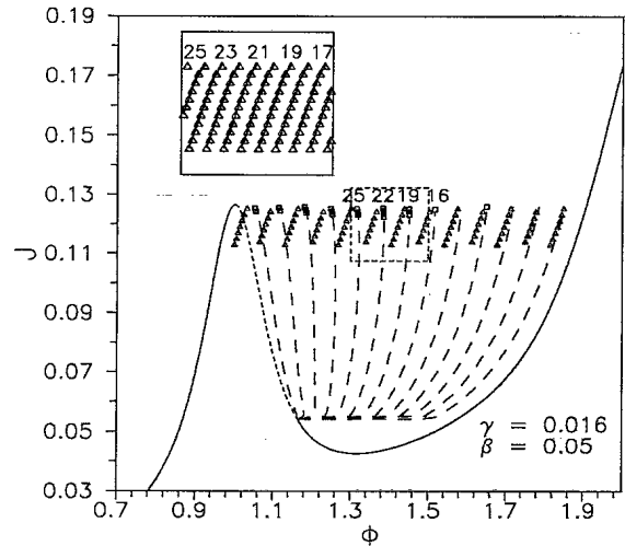
FIG. 3. Static characteristic curve: current ( J ) versus applied bias ( \phi ) for laser power \gamma = 0.016 ( \beta , which is only relevant for the stability of the different solutions [see (A2) in the Appendix], is assumed to be 0.05). The solid line corresponds to the stable uniform solution. In the NDR part of the curve there is a region where this solution becomes unstable (short-dashed line). The remaining curves correspond to two-domain solutions. There are 39 branches (one less than the number of quantum wells), though only one of every three branches has been plotted for the sake of clarity. The inset enlarges a small region of the figure showing the branches in full detail. Each branch has a different number of wells (from 1 to 39) in the low-field domain (the number written on top of some of them). Every branch consists of two curves, according to the way they are built with the discrete mapping (2.4) (see text for details): one plotted with triangles, corresponding to jumps from the first to the third fixed points of (2.4), and another plotted with a combination of squares (stable part) and long dashed lines (unstable part), corresponding to jumps from the second to the third fixed points of (2.4). Important features to stress from this figure are first, the coexistence, for a given \phi , not only of several domain solutions but also of domain solutions and the uniform solution (see also Fig. 5), something relevant to the appearance of hysteresis and memory effects, and second, the average “flatness” of J in the bias region between the two local maxima of v(E) .
