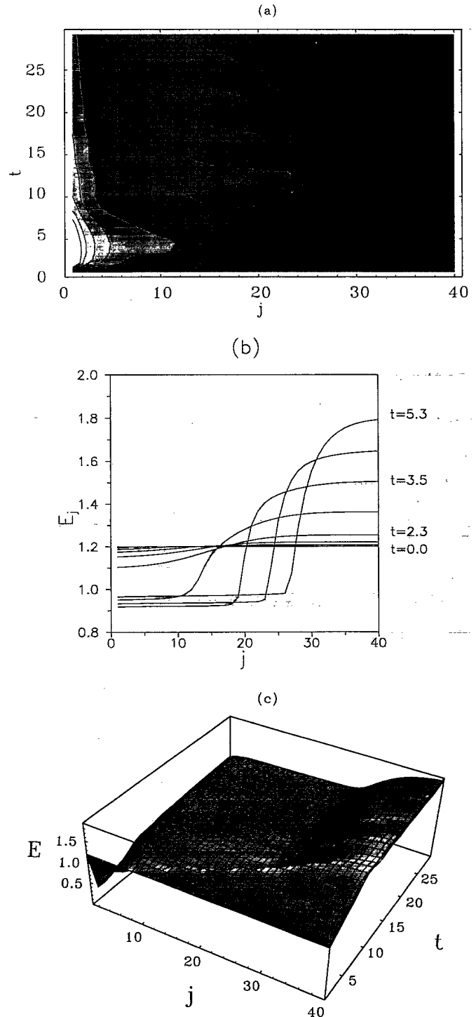
FIG. 6. Evolution of the domain wall in time for \gamma = 2 \times 10^{-3} and \phi = 1.2 . (a) is a contour plot with time flowing on the y axis and the quantum well number on the x axis. The electric-field contours go from 0.5 to 1.7 in 0.1 steps. At t = 0 we start with the uniform solution. The perturbation is clearly visible at the first well at short times. The creation and the displacement of the domain wall can be visualized. At t = 0.5 the two domains are already defined (the darker the figure the higher the electric field) and the domain wall begins to oscillate. Most of the wells have an electric field centered around the first maximum of v(E) (low-field domain). In (b) we represent the electric-field profile at short times (domain formation) and in (c) the domain wall oscillations.
