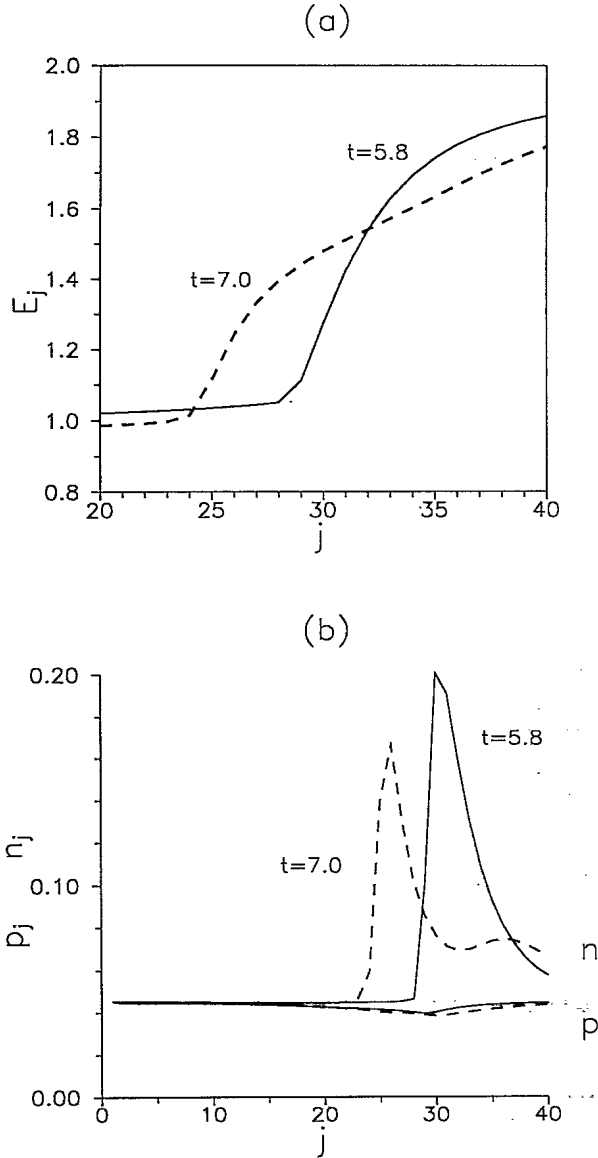
FIG. 9. (a) Electric-field profile and (b) charge at each well corresponding to a maximum (full line) and a minimum (dashed line) of the PC. Parameter values are the same as in Fig. 6.
