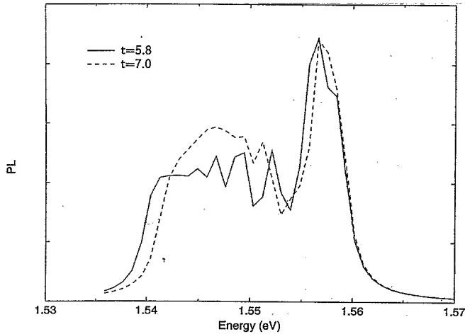
FIG. 10. Oscillations of the PL spectrum corresponding to Fig. 9.
