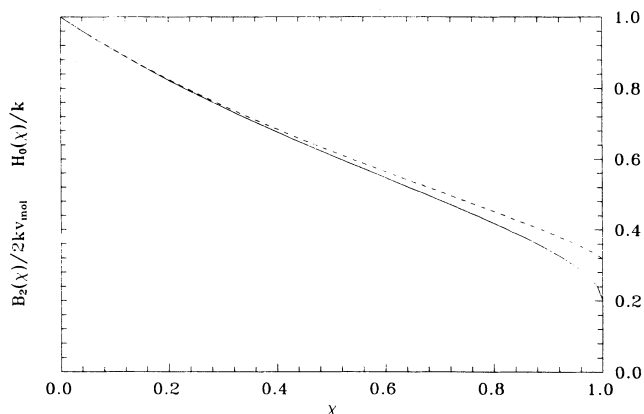
FIG. 4. Comparison between the exact second virial coefficient and the one obtained from the Gaussian-overlap approximation (see text). Solid line represents B_2(\chi)/2kv_{\text{mol}} , with B_2(\chi) given by Eq. (8), and dashed line represents H_0(\chi)/k , with H_0(\chi) given by Eq. (10); both curves are plotted against the eccentricity \chi \equiv (k^2 - 1)/(k^2 + 1) , k being the aspect ratio of the ellipses. The eccentricities [\chi(k)] of the three simulated cases are \chi(2)=0.6 , \chi(4)=0.882 , and \chi(6)=0.946 .
