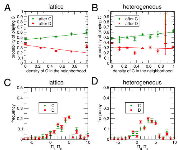
Fig. 3. Players' behavior depends both on the level of cooperation in the neighborhood and their previous action. Frequency of cooperative actions after a cooperative/defective action conditioned to the context (fraction of cooperative actions in the neighborhood in the previous round) observed in the lattice ( A ) and the heterogeneous network ( B ). Details of the linear fits and comparison with randomizations to prove statistical significance can be found in Table S2 and SI Results and Discussion . The plots show that there is a relevant dependence on the context for subjects who cooperated in the previous round (i.e., were in a cooperative mood): the cooperation probability increased with the fraction of cooperative neighbors, similar to the conditional cooperators found in the work by Fischbacher et al. (24). However, after having defected, this dependence is less clear, and if anything, it suggests an exploiting behavior—subjects who defected are less prone to cooperate the more cooperation they find. C and D show how subjects who cooperated or defected are distributed according to the largest payoff-per-link difference in their neighborhoods between the two actions. These plots reveal that a player's decision to cooperate or defect was independent of the payoffs per link that they observed (information that was explicitly provided during the experiment).
