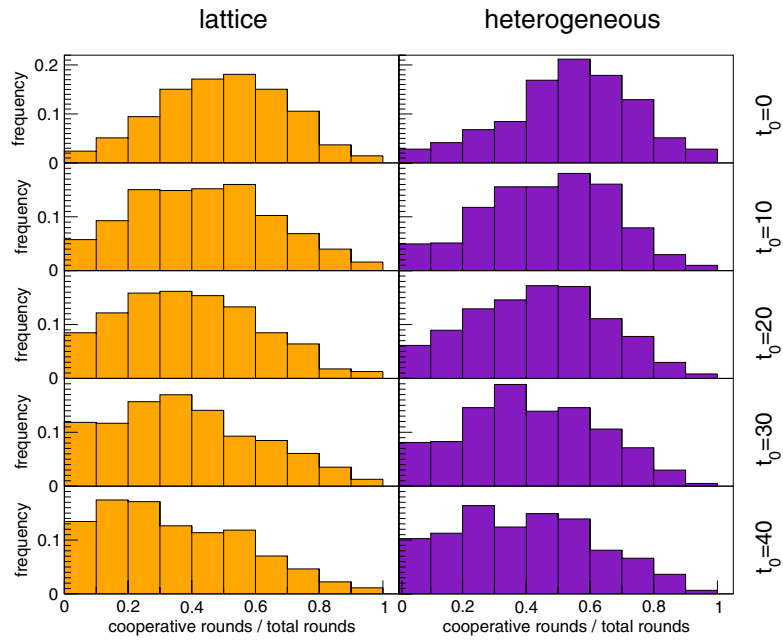
Fig. 55. Time evolution of the distribution of cooperative actions. The different panels show how frequently players cooperated in different time periods. The results correspond to the first treatment (experiment). Rows represent periods 1–10 ( t_0 = 0 ), 11–20 ( t_0 = 10 ), 21–30 ( t_0 = 20 ), 31–40 ( t_0 = 30 ), and 41–50 ( t_0 = 40 ) as indicated.
