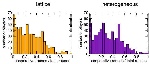
Fig. 54. Distribution of cooperative actions in the control. We represent the number of players that cooperated during the given number of rounds (normalized by the total number of rounds played). The results correspond to the control phase. Similar results were presented in Fig. 2.
