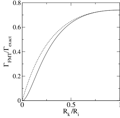
Figure 2. The ratio between \Gamma_{\text{FMT}}^{(3)} = 4\pi^4 R_i^2 R_j^2 R_k^2 and \Gamma_{\text{exact}}^{(3)} (equation (2.2)) for R_j = R_i \geq R_k (solid curve) and for R_j = R_i \leq R_k (dashed curve).
